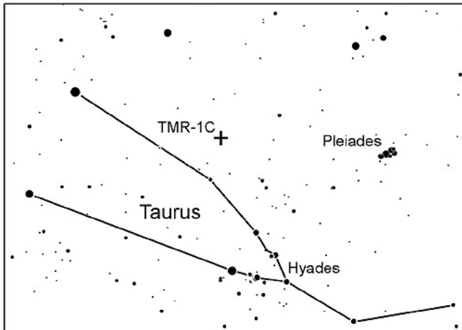
Location of Protoplanet TMR-1C on the Sky
